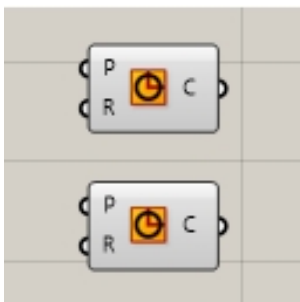
Grasshopper Canvas
